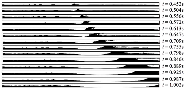
Fig. 4 slug modeling at 12 m/s velocity difference
