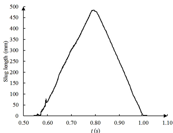
Fig. 12 Slug length
