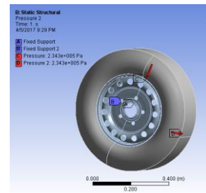
Fig. 11 Rim and tire loading and boundary conditions in modal and static analysis
