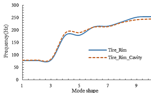
Fig. 23 Comparison of the results of modal analysis for tire and rim model compared with tire, rim and acoustic fluid cavity model
