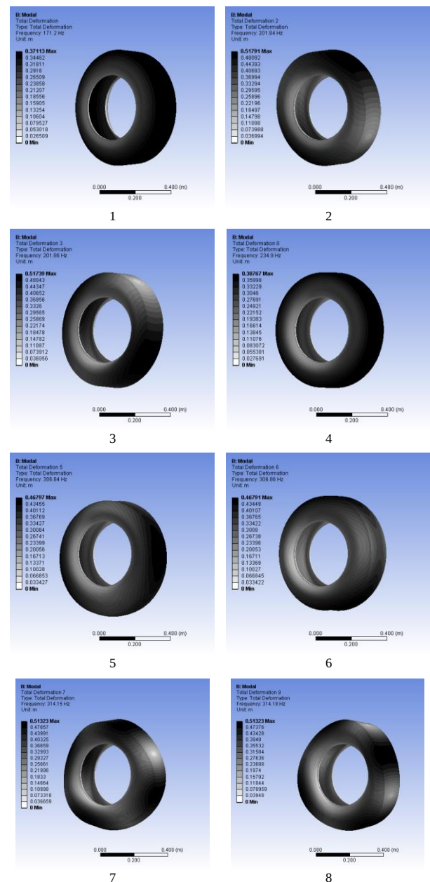
Fig. 16 The first eight natural frequencies and modes of tire model
