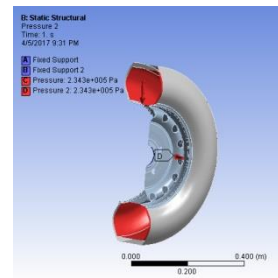
Fig. 11 Rim and tire loading and boundary conditions in modal and static analysis
