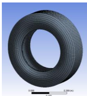
Fig. 8 Mesh of tire structural model
