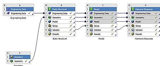
Fig. 14 Coupling harmonic analysis with static and modal analyses
