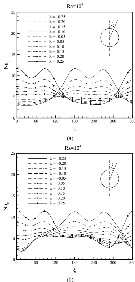
Fig. 5 Distribution of local Nusselt number along the surface of the inner cylinder ( Nu_c )
