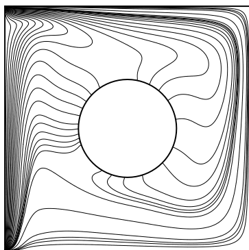
Fig. 2 Isotherms around the isolated cylinder at Ra=10^6
