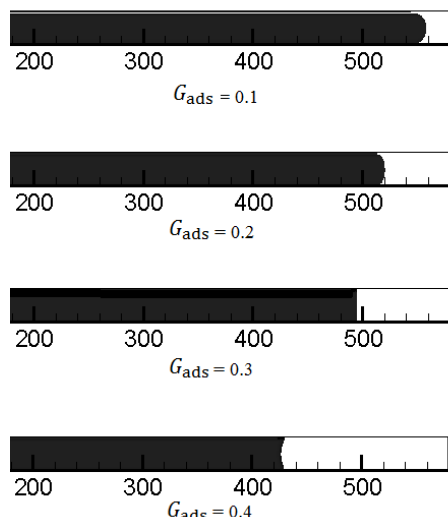
Fig. 8 The obtained result for the two-phase flow in channel with hydrophobic and hydrophilic surface at the time t = 2000\text{ls} after initial condition for different values G_{\text{ads}}
