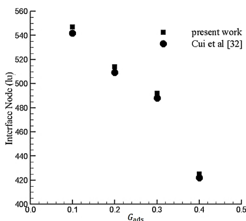
Fig. 9 The contact area location of the phase 1 and 2 at the time t = 2000\text{ls} based on different values G_{\text{ads}} and compared with the results obtained by Jing Cui et al. [32]
