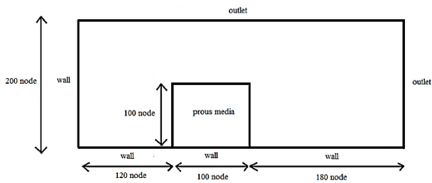
Fig. 5 The problem boundary condition
