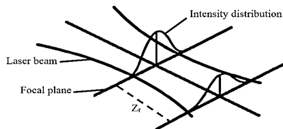
Fig. 4 Schematic of laser beam gaussian distribution
