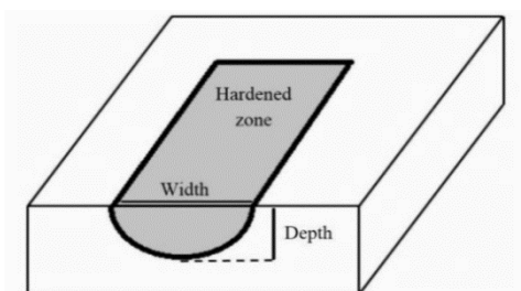
Fig. 1 Schematic of geometrical dimensions of hardened zone (width and depth)
