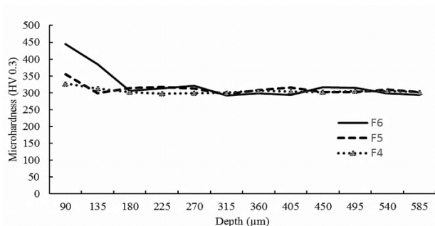
Fig. 6 Microhardness profile in depth of the laser hardened layer in focal point position tests
