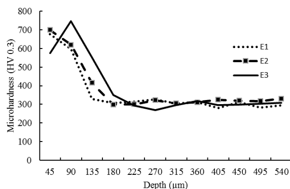
Fig. 7 Microhardness profile in depth of the laser hardened layer in laser pulse energy tests
