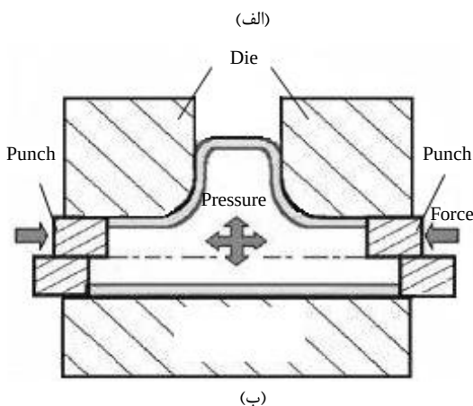
Fig.6 (a) Experimental setup of T-shape Hydroforming (b) A schematic of setup of T-shape Hydroforming
