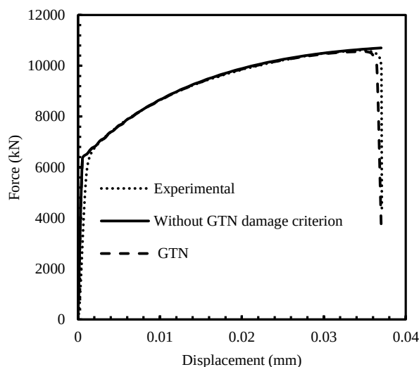
Fig. 8 Force – displacement curve of tension test specimen
