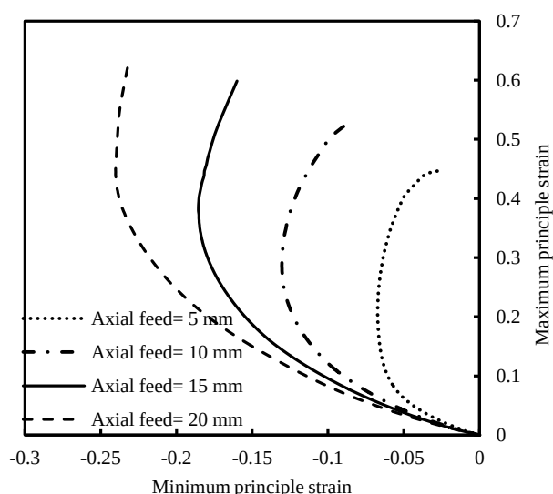
Fig. 17 Effect of axial feed on strain path (bulge length of 60 mm and die radius of 5 mm)
