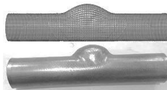
Fig. 28 Comparison bulging parts in experimental and FEA
