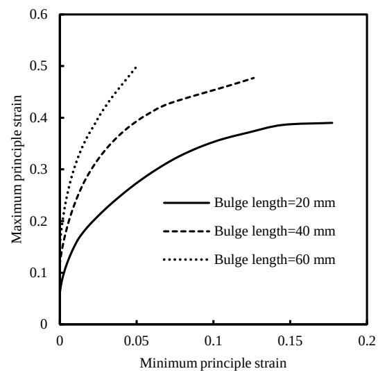
Fig.15 Strain path with respect to bulge length in free bulge test
