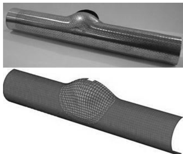
Fig. 23 Predicted fracture in experimental and FEM by entering the coefficients GTN
