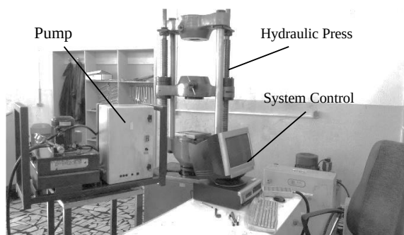
Fig. 4 Universal testing machine and hydraulic pressure unit
