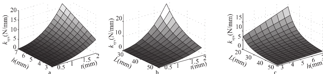
Fig. 7 Parametric effects of thickness, height and length of the beam flexures on the proposed compliant mechanism stiffness
