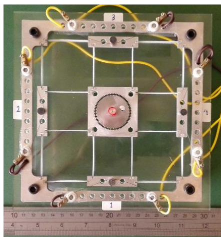
Fig. 10 Fabricated prototype of SMA wire drive wobble motor
