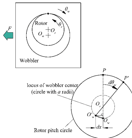
Fig. 4 Amount of contact point rotation due to differential motion of wobbler
