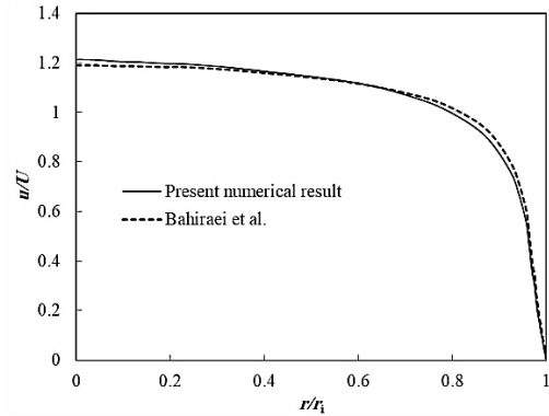
Fig. 4 The results of current numerical method in comparison with the results of Bahiraei et al
