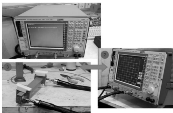
Fig. 11 1) Front view of Device 2) The device is ready for measurement 3) Putting samples in waveguide and measuring the amount of absorption
