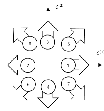
Fig. 3 Curvature change directions on C^{(1)} - C^{(2)} plane
