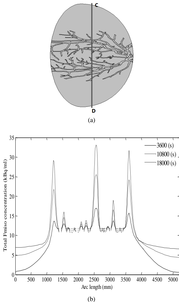
Fig. 13 (a) The exhibition of solid cut line CD (b) The curve of total Fmiso concentration ( \frac{kBq}{ml} ) across this line for different time steps
