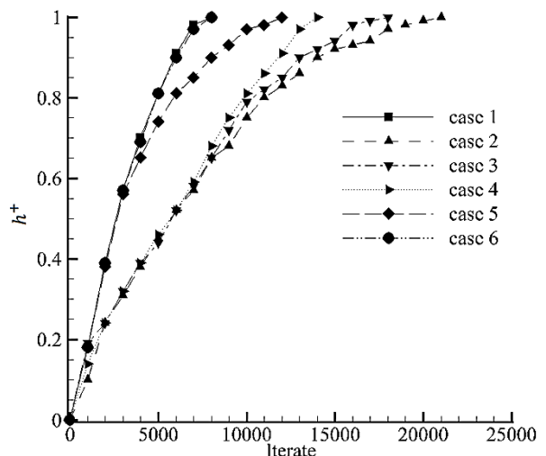
Fig. 14 Penetration of fluid in porous medium for different states
