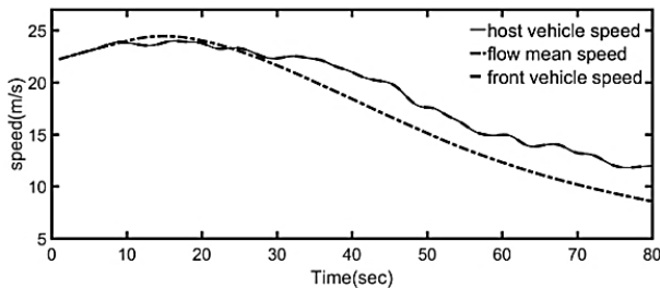
Fig. 13 First maneuver: Tracking target vehicle to check accuracy of adaptive cruise control
