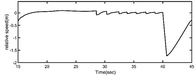
Fig. 24 Relative speed control in the third maneuver
