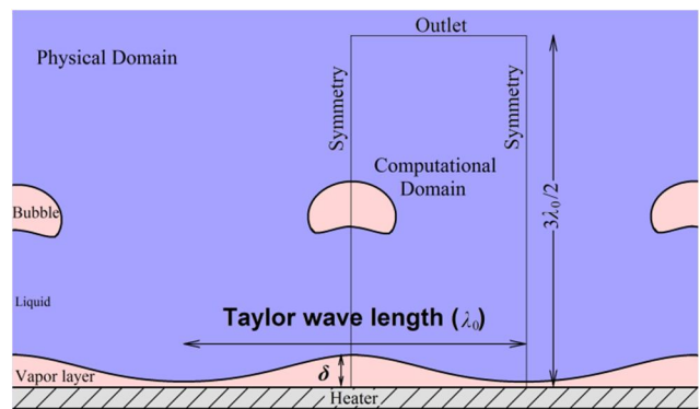
Fig. 1 Geometry and boundary conditions of film boiling
