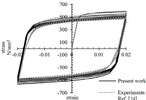
Fig. 13 Comparisons between the predictions from the cyclic material model in the current study with the cyclic coupon test data from [24]
