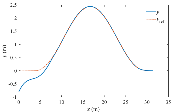
Fig. 4 The lateral trajectory of the trailer
