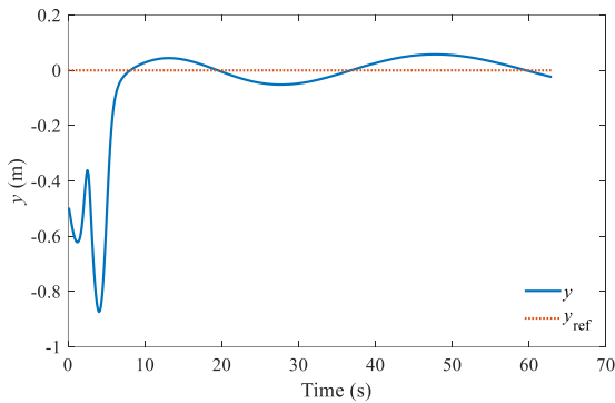
Fig. 13 The lateral trajectory of trailer in the caresian coordinate
