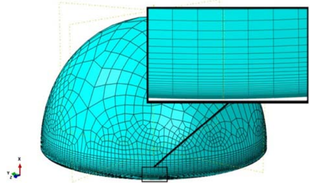
Fig. 3 Model meshing
