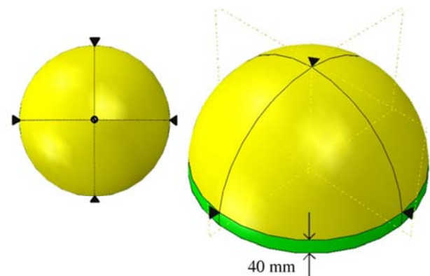
Fig. 4 Mechanical constraints
