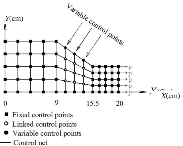
Fig. 15 Design variables for two-dimensional fillet example
