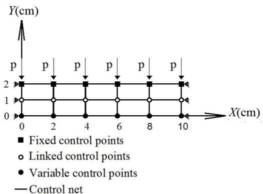
Fig. 19 Initial design of a clamped beam
