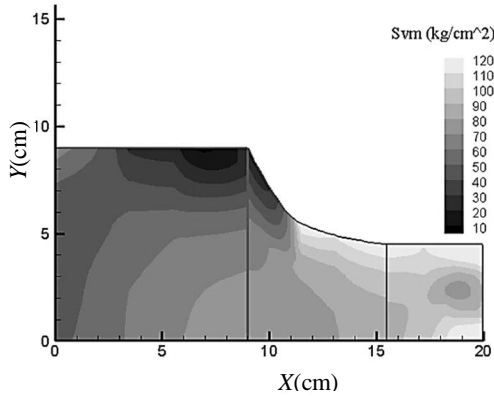
Fig.17 von Mises stress Contours and optimum boundaries
