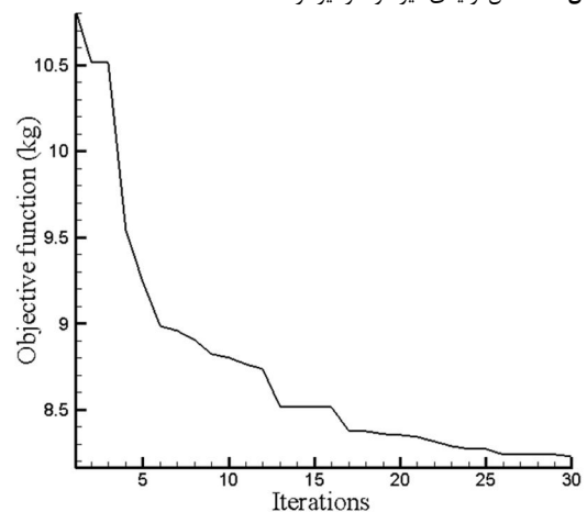
Fig. 20 Iteration history for the clamped beam
