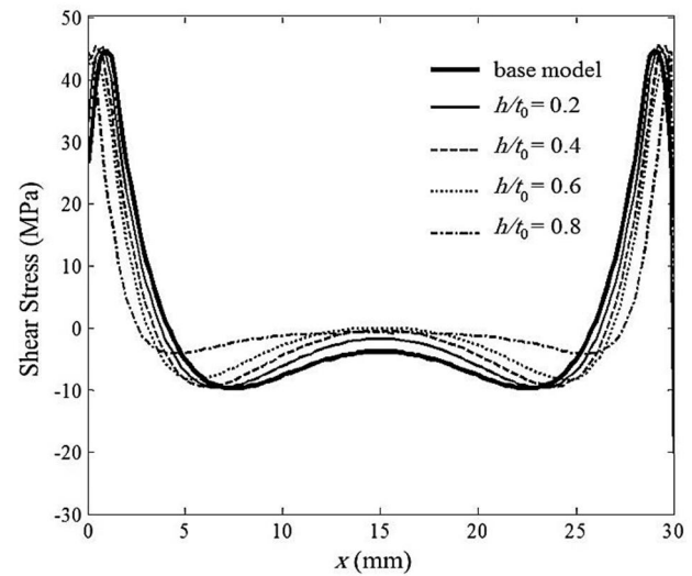
Fig. 11 effect of tapered adherend on shear stress in overlap length
