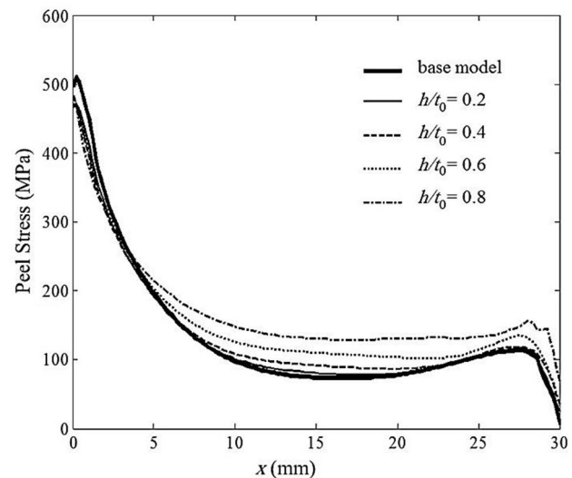
Fig. 12 effect of tapered adherend on peel stress in overlap length
