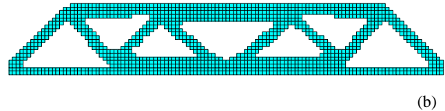
Fig.8 Optimal topology for beam with ER = 2%:
