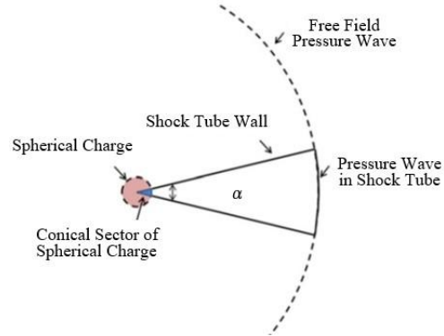
Fig. 1 Amplifying the explosive charge in a conic shock tube [1]
