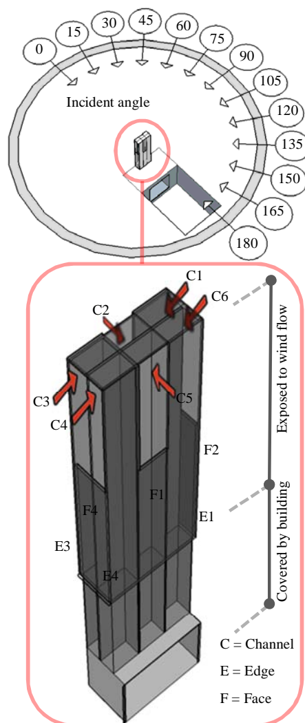
Fig. 9 wind incident angels and naming windcatcher details
