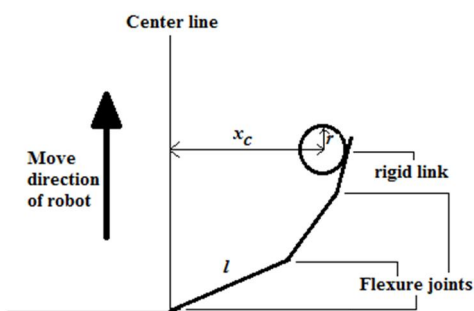
Fig. 4 The contact of object on the distal link
