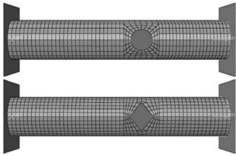
Fig. 9 Meshing figure of shells
