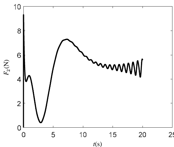
Fig. 5 - b F_2 propeller force in presence of uncertainties and without identification
