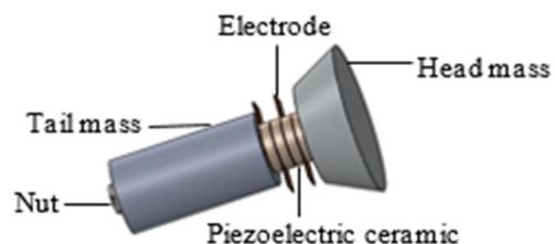
Fig. 6 Schematic view of the designed transducer
