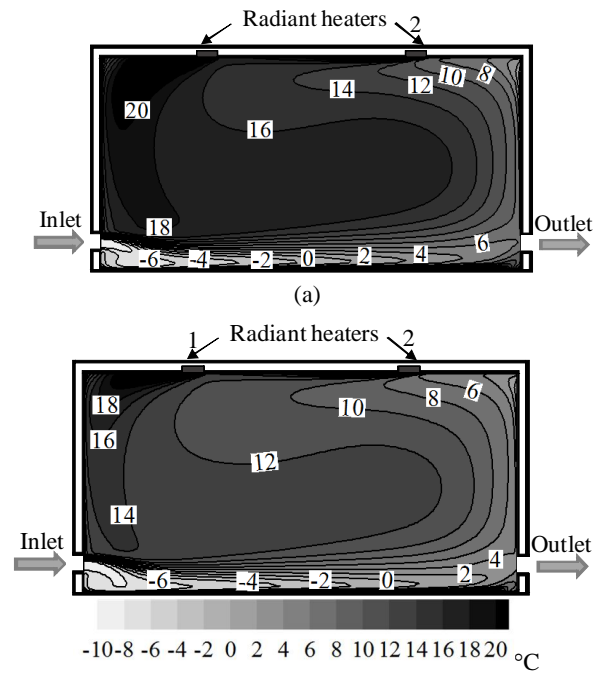
Fig. 8 Air temperature contours in chamber with couple radiant heaters for (a) 5 air changes per hours, (b) 10 air changes per hours
