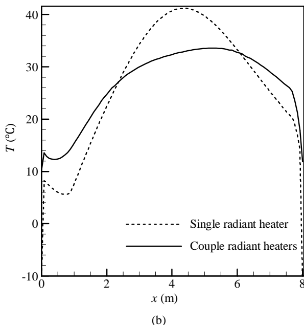
Fig. 9 Temperature distribution of floor of hall for (a) 5 air changes per hours, (b) 10 air changes per hours
