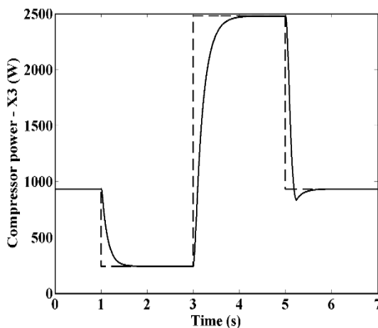
Fig. 8 Compressor power for sliding mode controller
