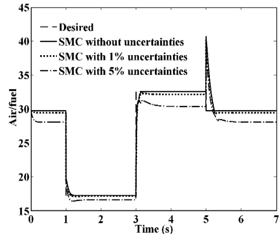
Fig. 11 Air fuel ratio based on changing the uncertainties value for sliding mode controller
