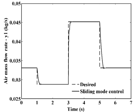
Fig. 9 Air mass flow rate for sliding mode controller
