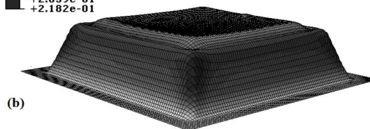
Fig.17 The predicted thickness distribution of the first strategy: a) the first stage b) the second stage
