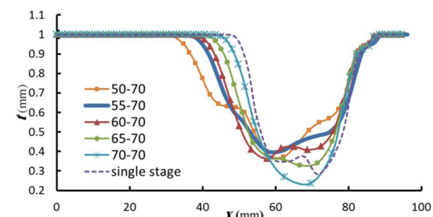
Fig.14 The predicted thickness distributions along path 1 based on Table 4
