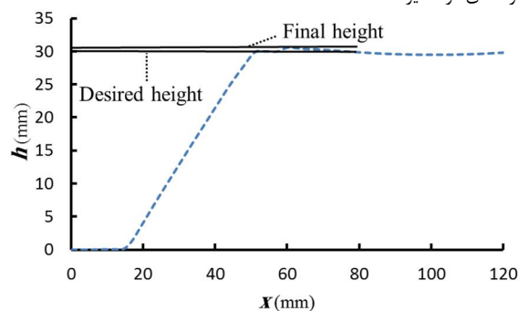
Fig.21 The predicted profile of the truncated pyramid with the 70 wall angle for Case 2 of the second strategy
