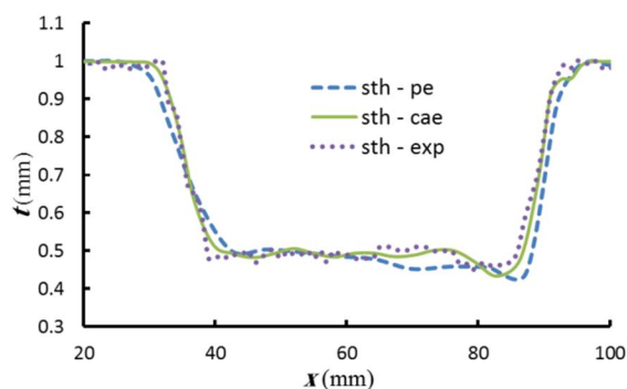
Fig.11 The comparison of thickness distribution for case 1 in path 1
