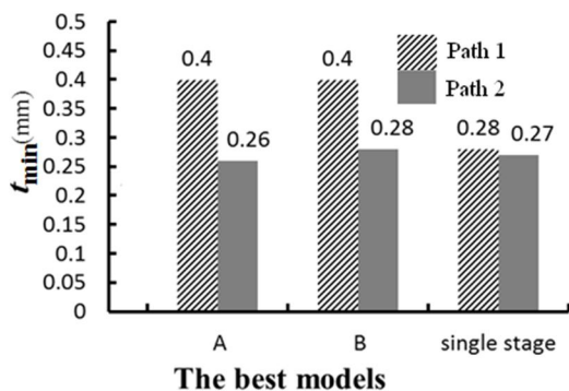
Fig.23 The comparison of the minimum thickness in single and two-stage strategies along Path 1 and 2
