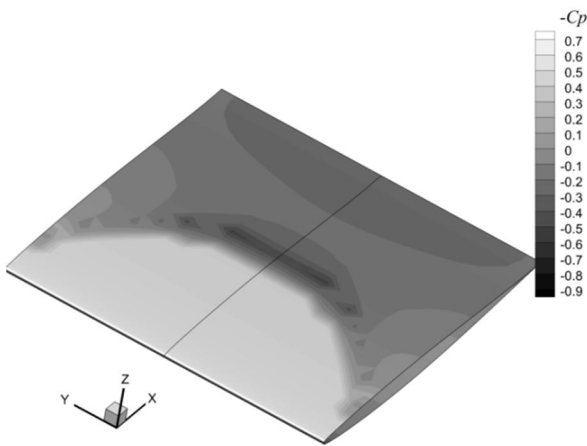
Fig. 13 Pressure distribution over the 3D wing with NACA16206 section at \alpha = 6^\circ , \sigma = 0.628
